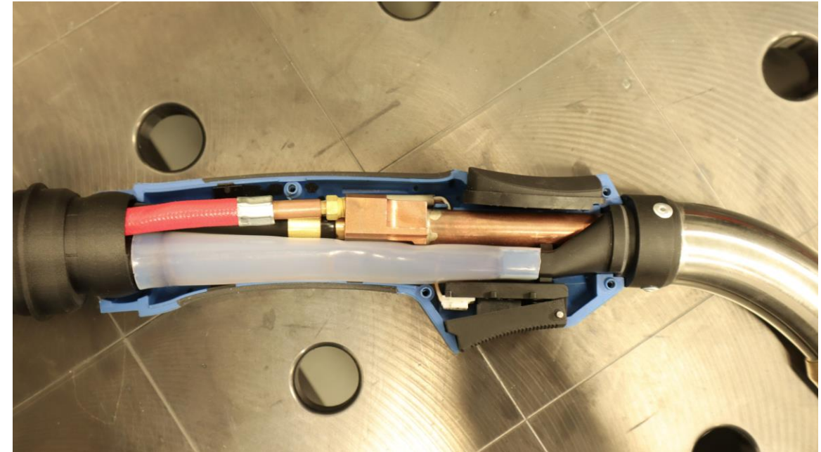
AiR WeldGuard fume extraction torch
